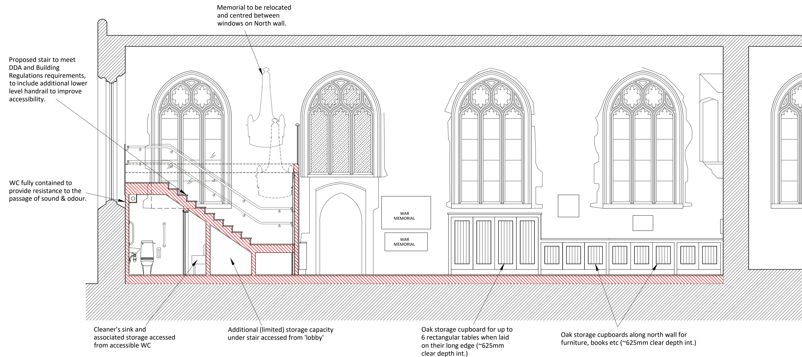
SECTION E-E
