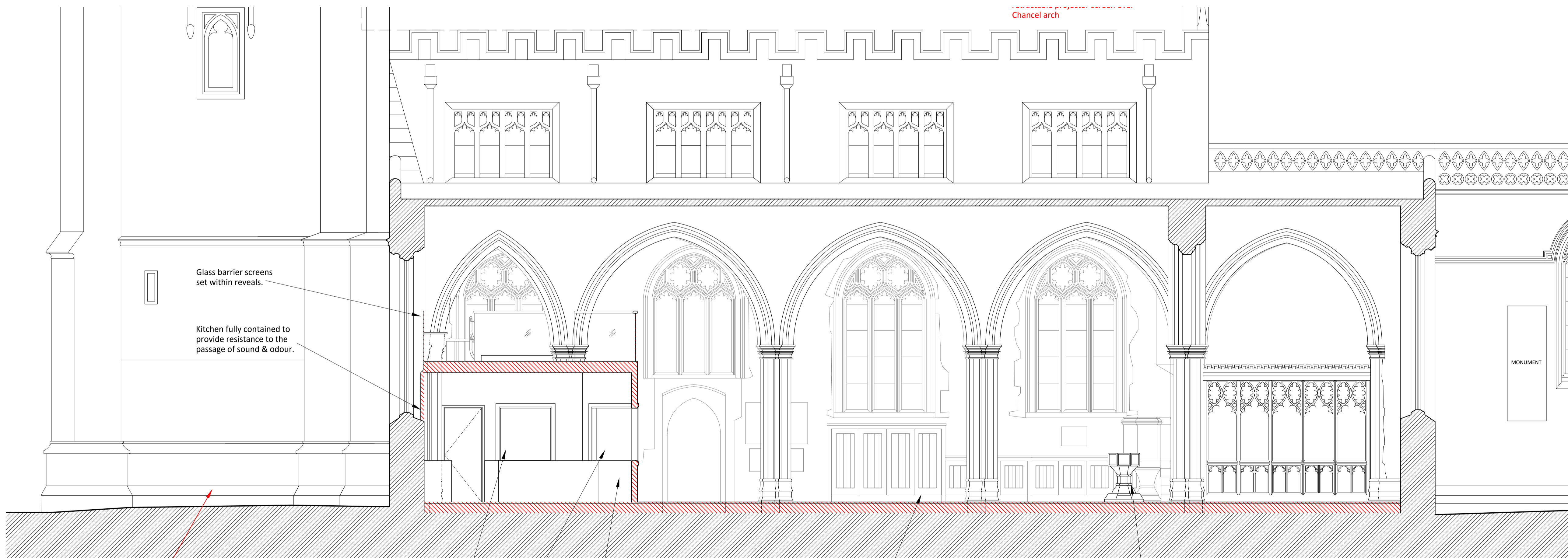
SECTION E-E
