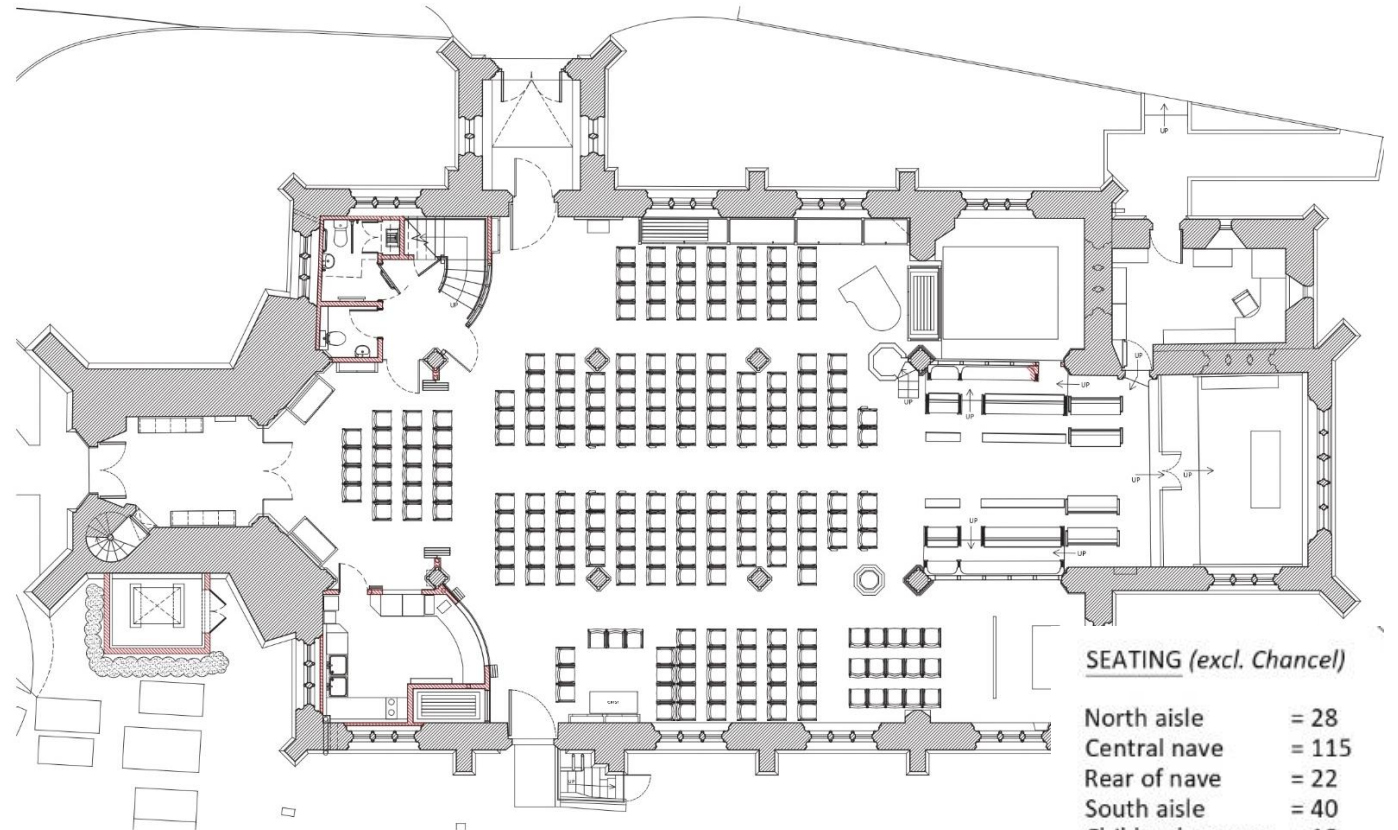
Ground Floor Plan Seating Option 1A - Traditional East Facing ( capacity )
