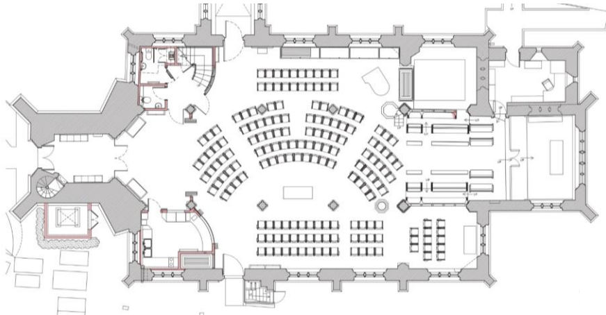
Ground Floor Plan Seating Option 2 - North-South Orientation
