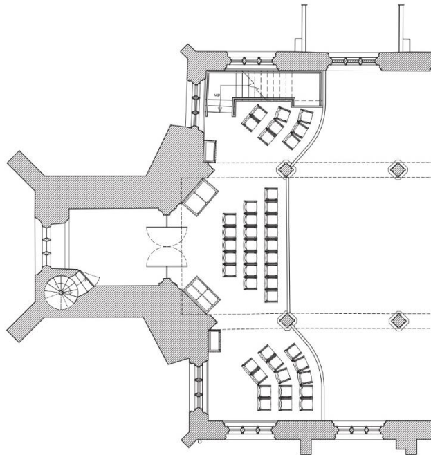
First Floor Plan Seating Option 1A
